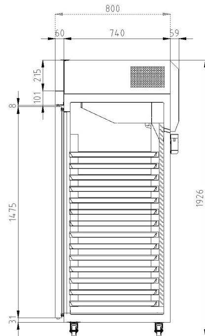
SIDE VIEW LONG DOOR
