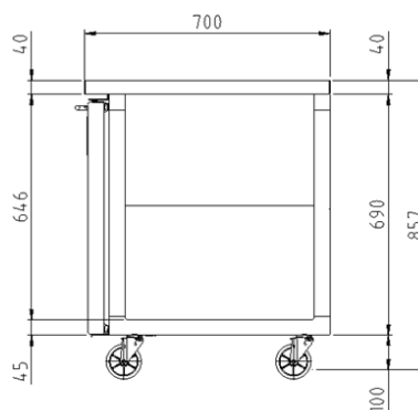
SIDE VIEW (Depth 700mm)
